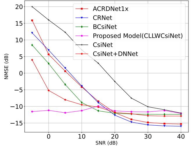
Fig. 3: Performance of Models under the various noise power and compression ratio of 8
