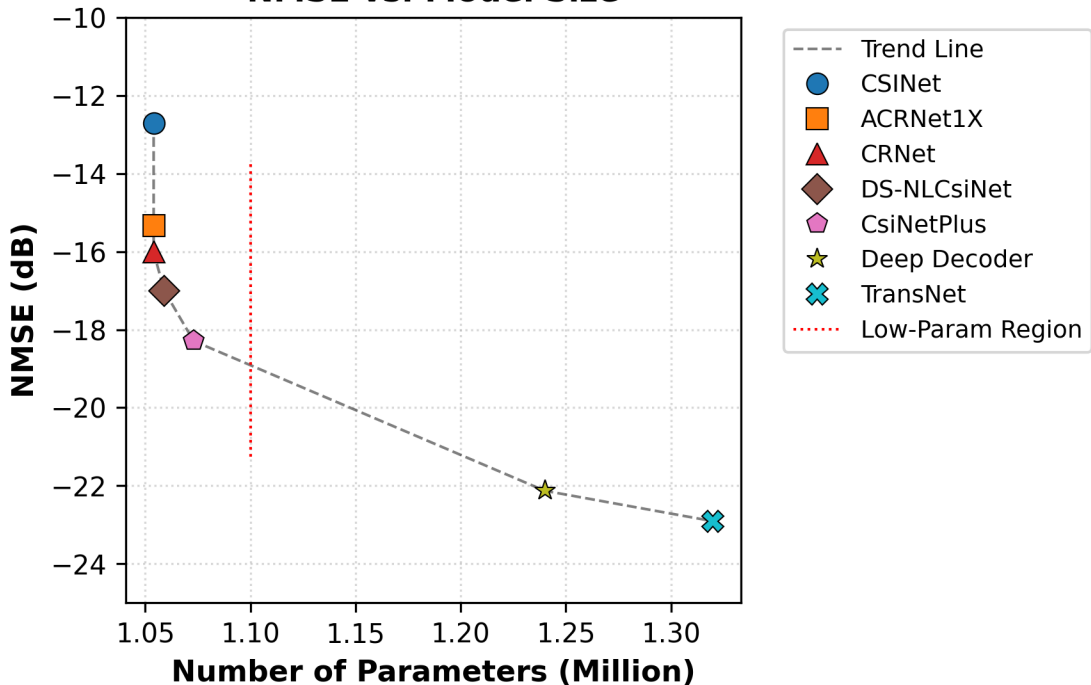
NMSE vs. Model Size
