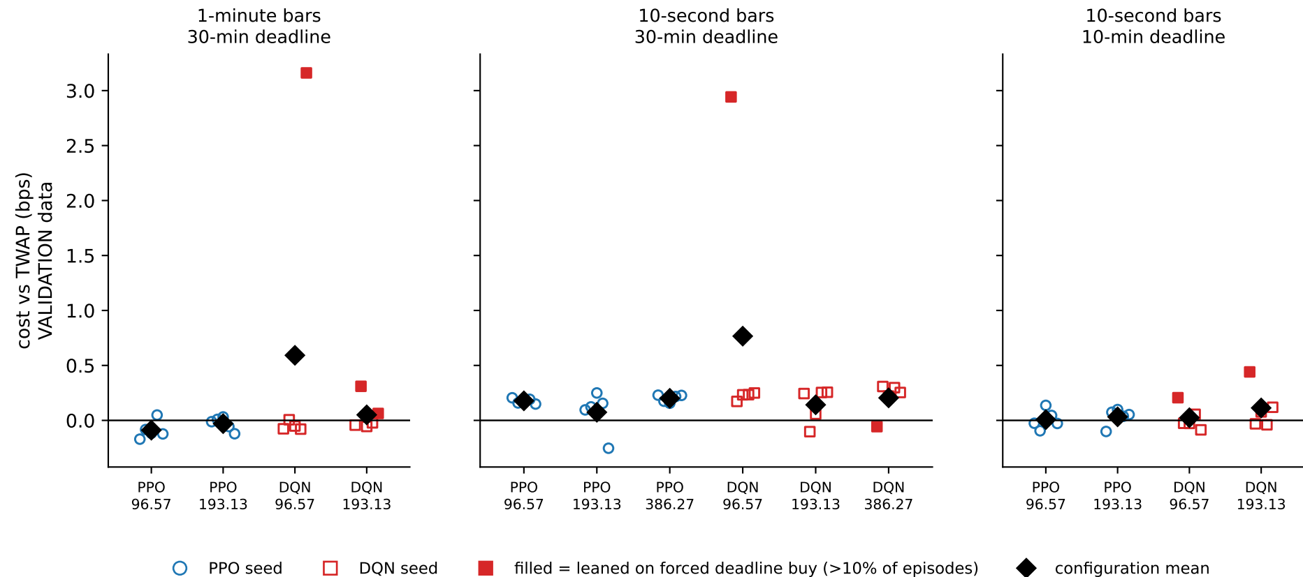
Recorded order books: cost against TWAP by bar resolution, order size and deadline, on validation data (all 70 agents)
