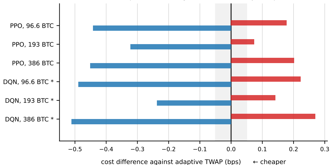
B. Every configuration on the affected dataset version, on validation and on the held-out test period, including three behaviourally collapsed
