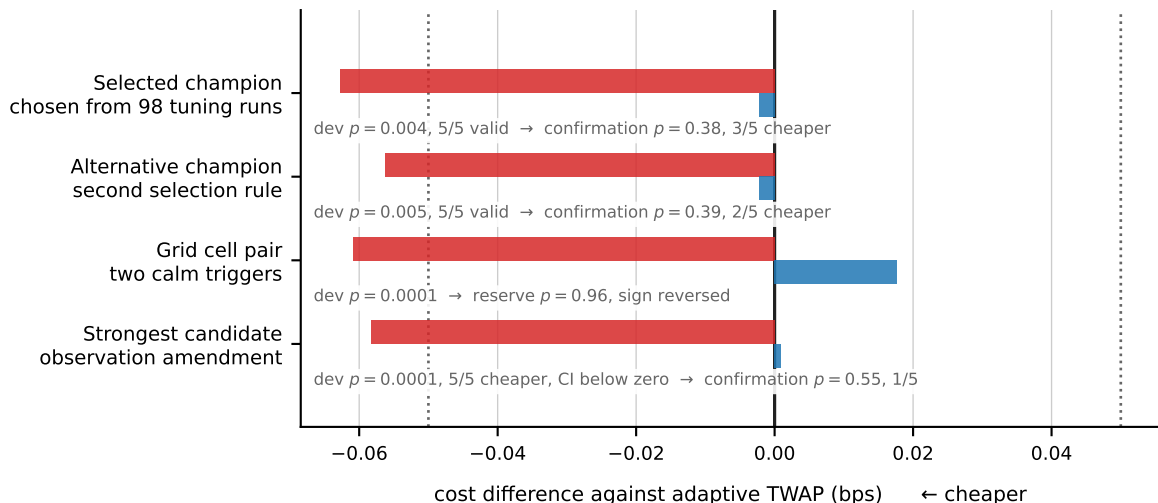
A. Four candidates, on the block each was found on and on a held-out block
