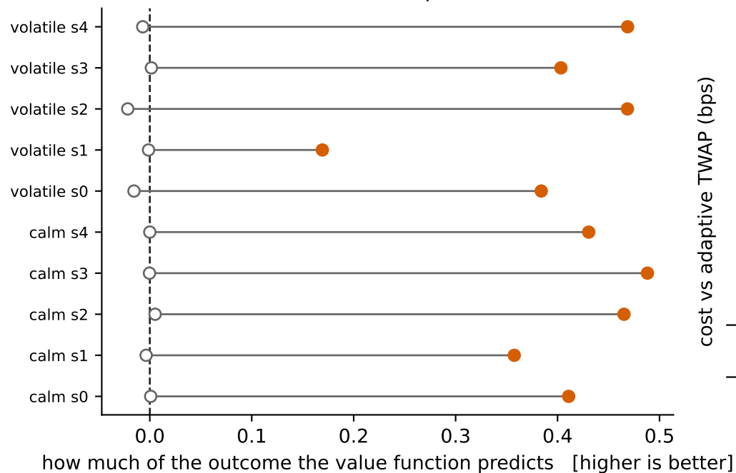
How well the value function predicts the outcome
