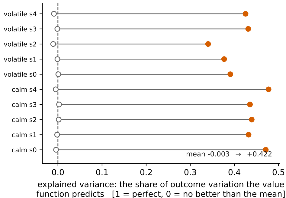
How well the value function predicts the outcome
