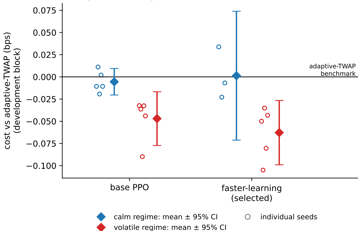
Cost against adaptive TWAP by regime, two configurations (development block; per-seed values with 95% confidence intervals)
