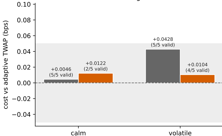
Execution cost against TWAP
