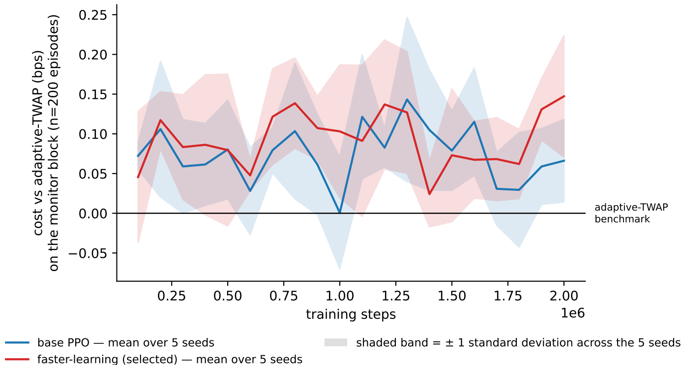
Training curves, volatile regime
