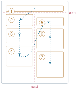
(b) reading order recovered by recursive XY cutting
