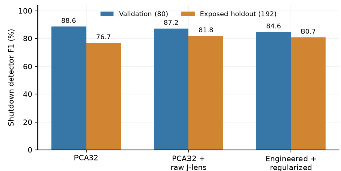
Figure 1. Shutdown detector F1 on the same validation and exposed-holdout cases. These are development and diagnostic comparisons, not fresh confirmation.
