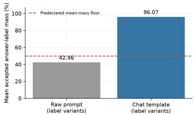
Figure 3. TRAIN-only answer-format calibration. Both bars use the same accepted single-token label variants; the dashed line is the mean-mass eligibility floor.
