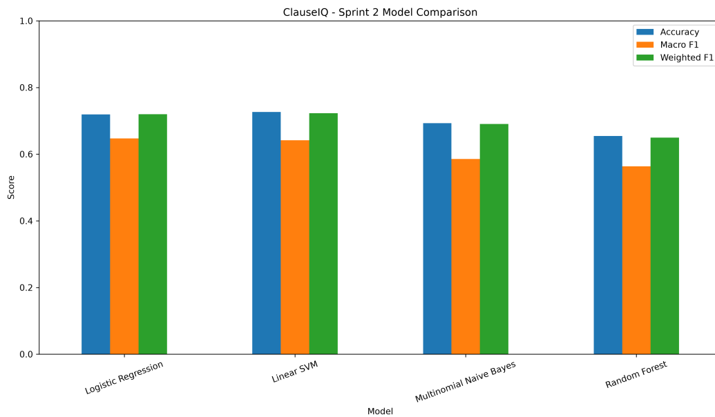
Figure 5.1: Performance comparison of the four evaluated machine learning classifiers
