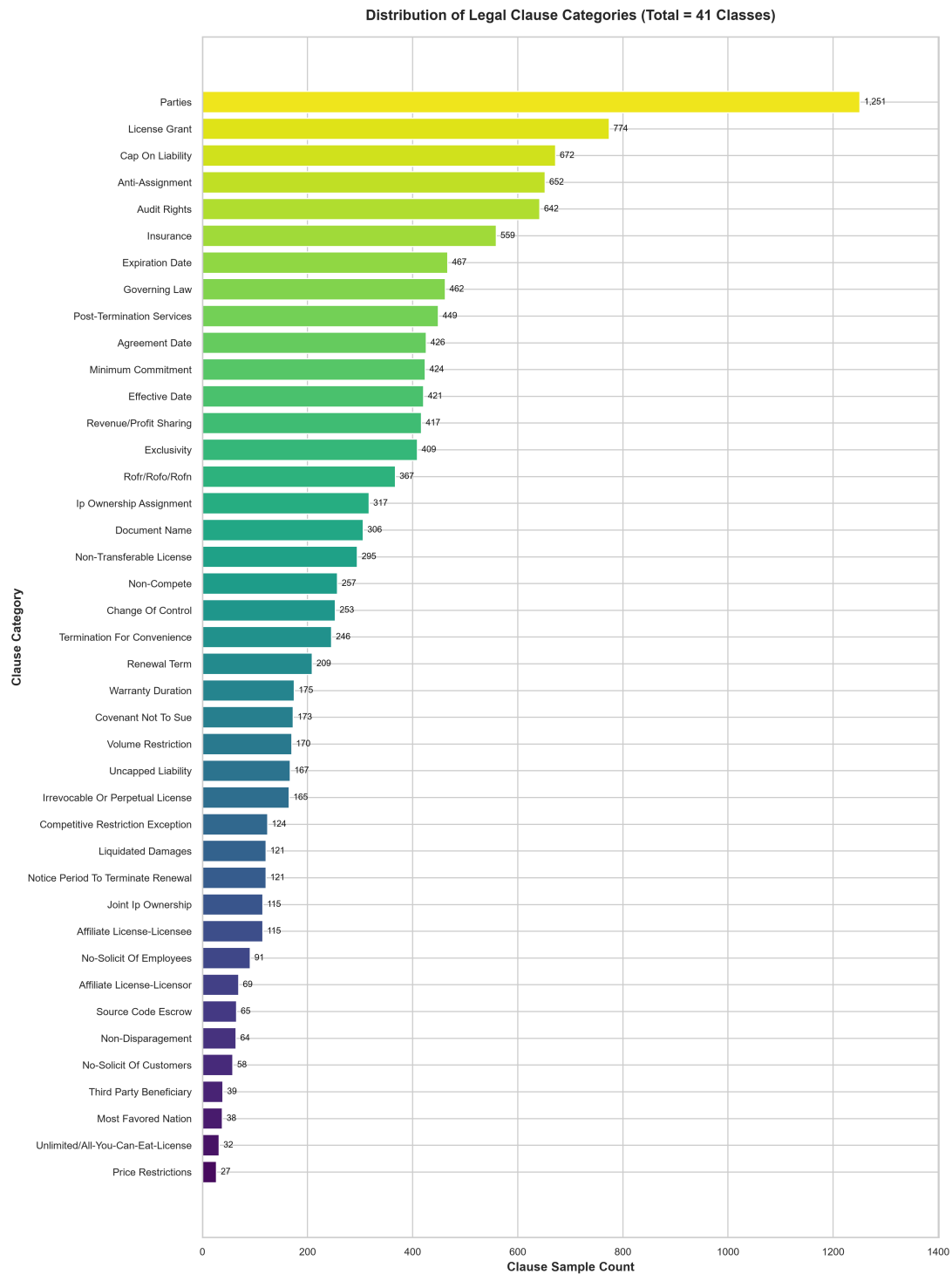
Figure 3.2: Complete 41-category class distribution in the ClauseIQ dataset ( N = 12,204 )
