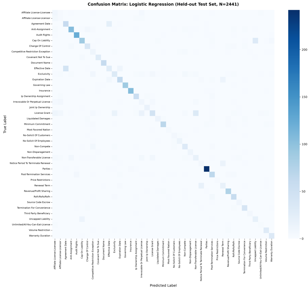
Figure 5.2: Full 41 \times 41 confusion matrix for the selected Logistic Regression model
