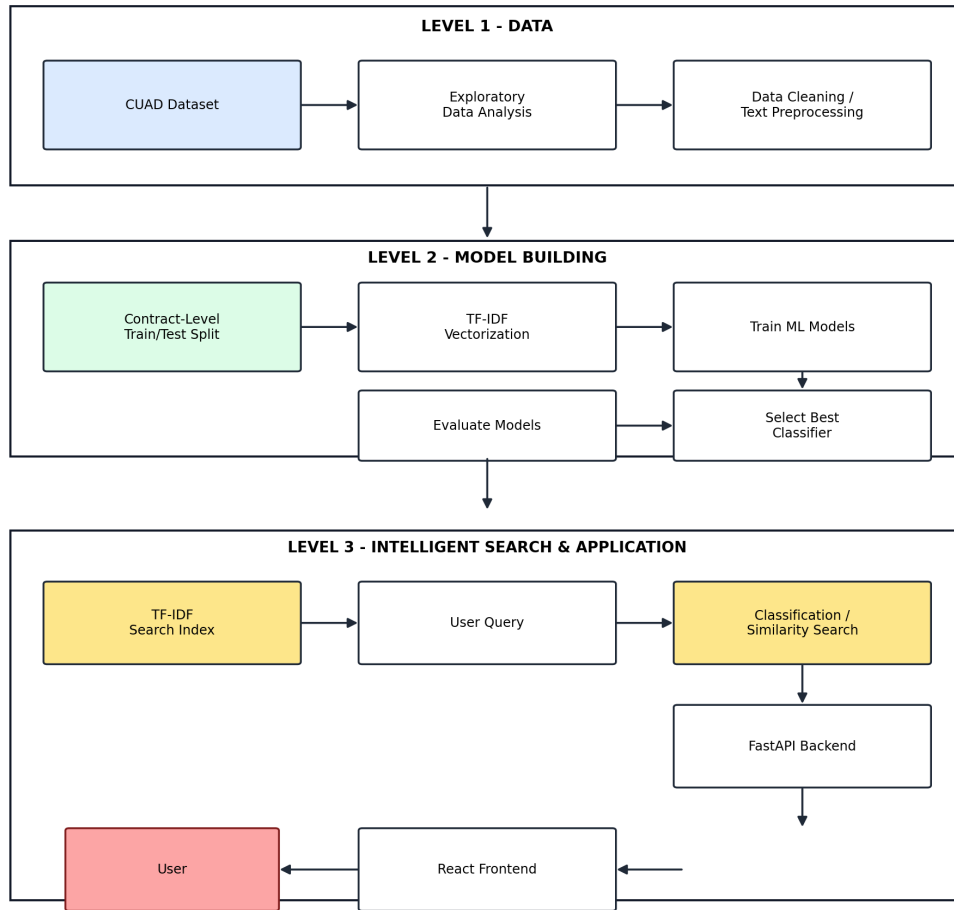
Figure 3.7: End-to-end ClauseIQ system pipeline architecture
