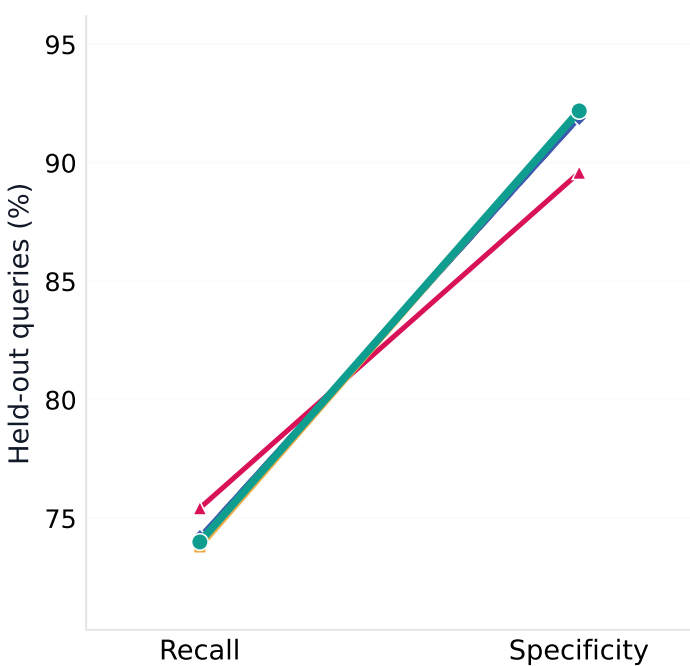
Idefics2-8B
