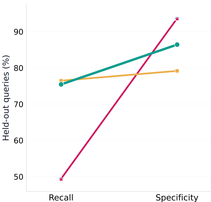
Idefics2-8B
