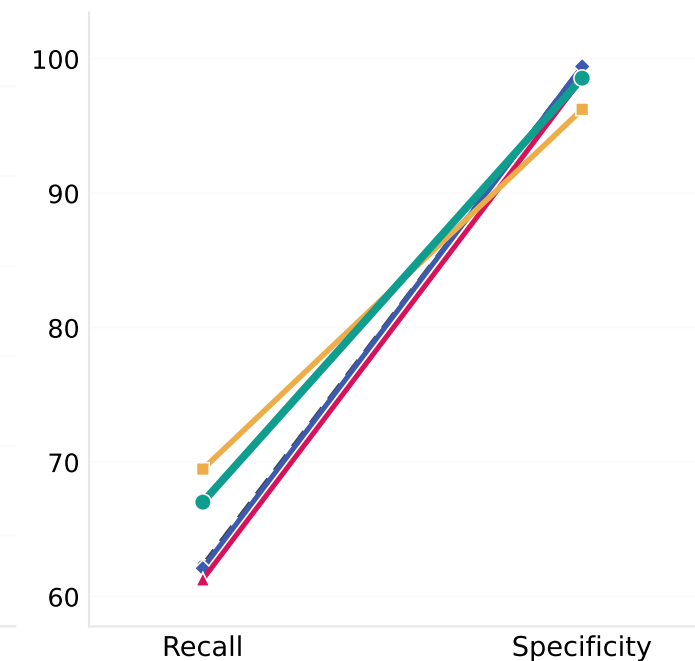
Qwen2.5-VL-7B
