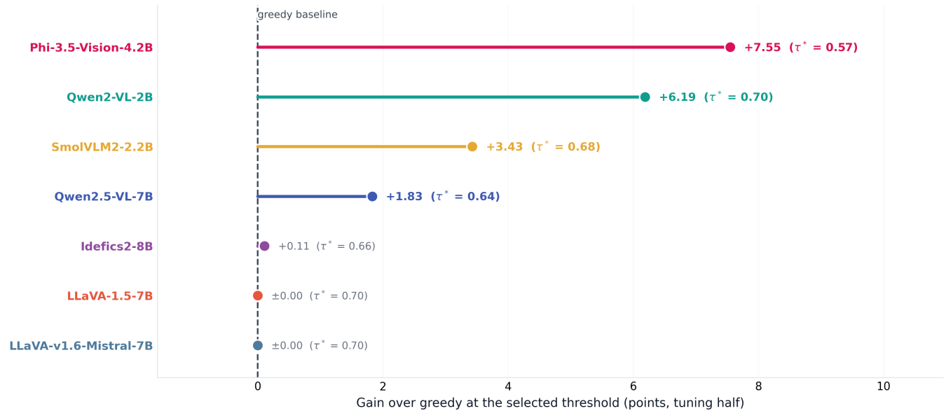
FIGURE 9. Gain over greedy decoding at each model's selected threshold \tau^* on the tuning half: the gate buys the most exactly where hallucination bias is largest.
