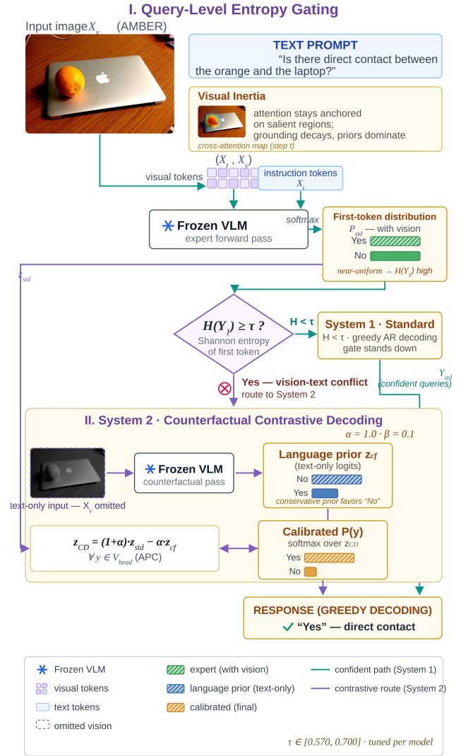
FIGURE 1. Overview of Entropy-Gated Contrastive Decoding (schematic). A relational query enters the frozen VLM; the first-token entropy H(Y_1) is compared against \tau , and the query is routed to System 1 (greedy decoding) or System 2 (counterfactual contrastive decoding with APC; \alpha = 1.0, \beta = 0.1 ). The selected-threshold interval across the seven evaluated models is \tau^* \in [0.570, 0.700] ; the search grid is [0.550, 0.750] .
