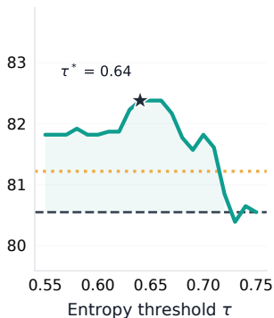
Qwen2.5-VL-7B
