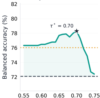
SmolVLM2-2.2B
