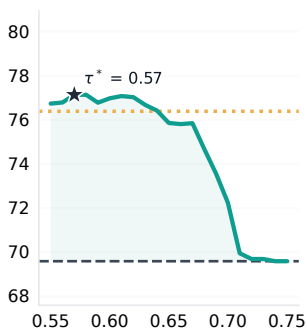
Qwen2.5-VL-7B
