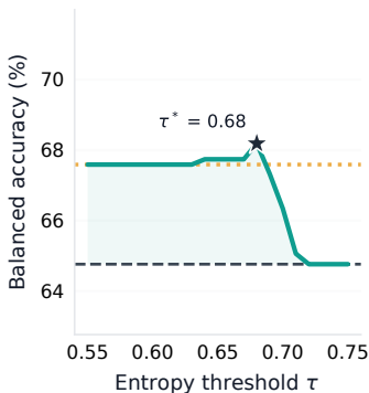
SmolVLM2-2.2B
