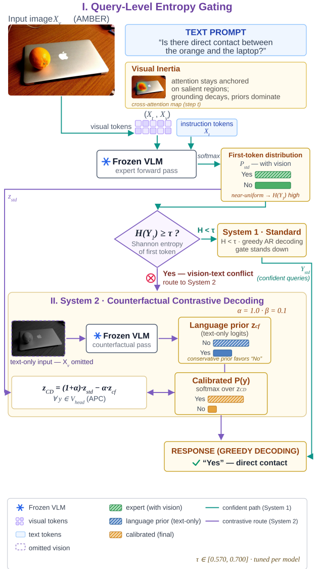
FIGURE 1. Overview of Entropy-Gated Contrastive Decoding (schematic). A relational query enters the frozen VLM; the first-token entropy H(Y_1) is compared against \tau , and the query is routed to System 1 (greedy decoding) or System 2 (counterfactual contrastive decoding with APC; \alpha = 1.0, \beta = 0.1 ). The selected-threshold interval across the seven evaluated models is \tau^* \in [0.570, 0.700] ; the search grid is [0.550, 0.750] .
