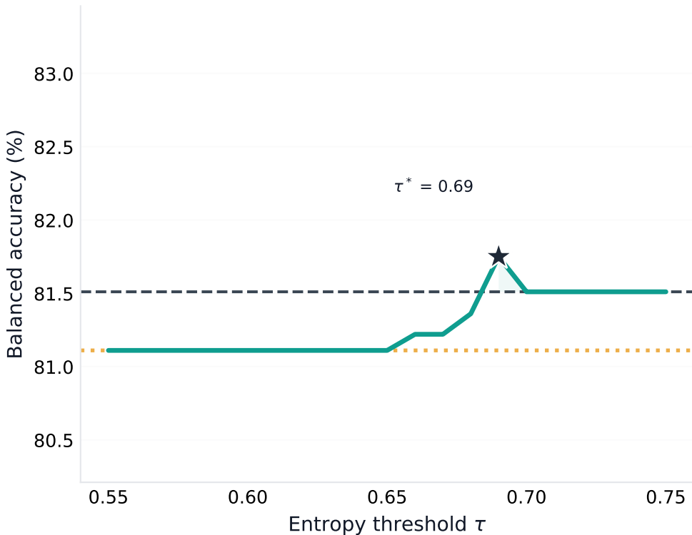
Idefics2-8B
