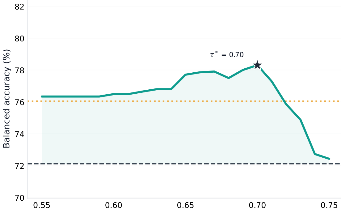
SmolVLM2-2.2B
