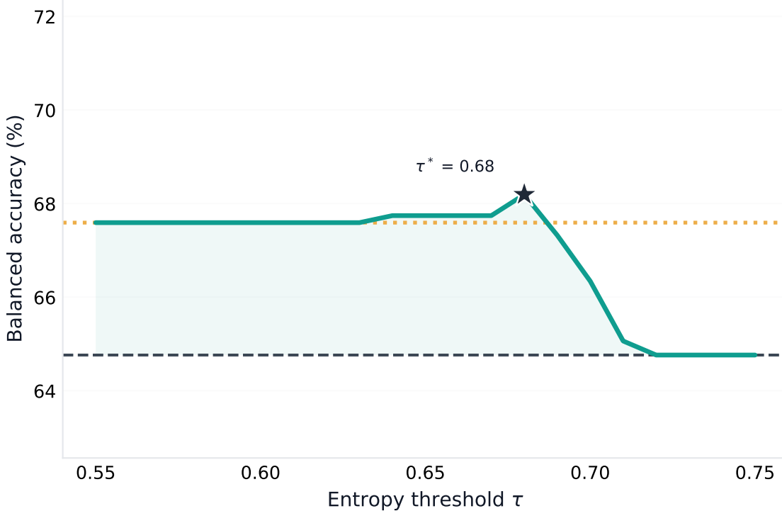
SmolVLM2-2.2B
