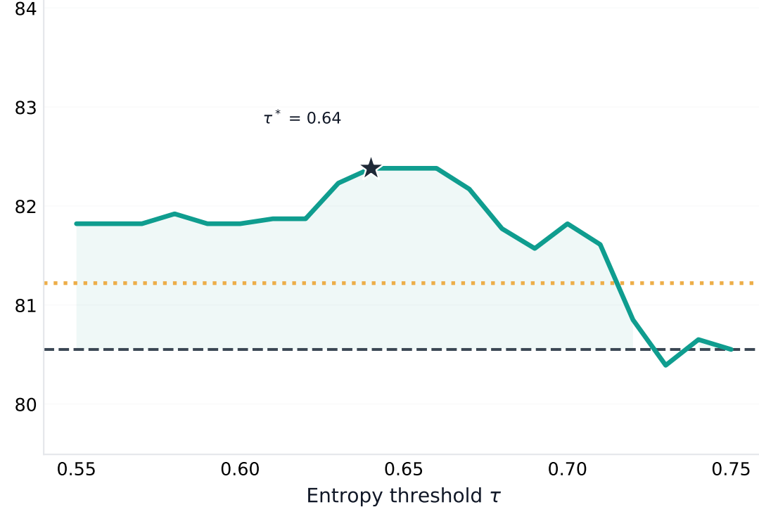
Qwen2.5-VL-7B
