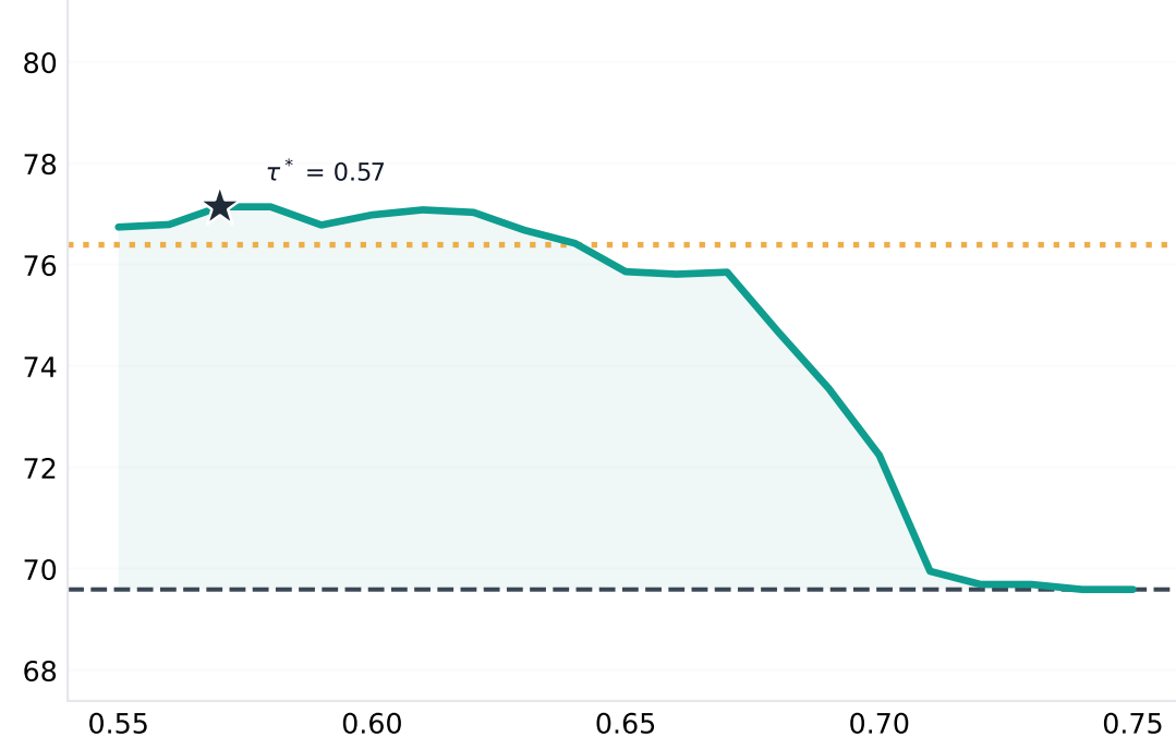
Qwen2.5-VL-7B
