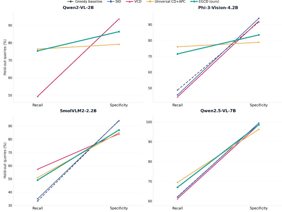
Fig. 4 Recall and Specificity on the held-out half for the four bias-affected models, where Universal CD+APC buys its recall by spending specificity and EGCD recovers most of the recall at a fraction of the specificity cost.
