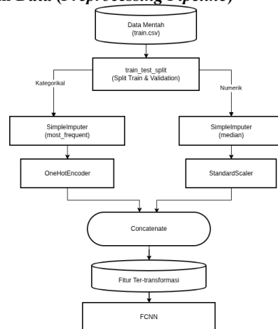
Gambar 4.10 Preprocessing Pipeline
