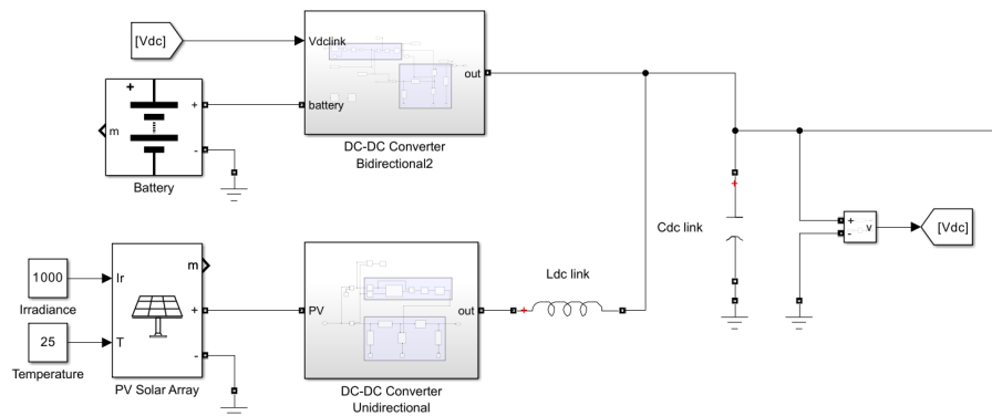
Gambar 3.1. Diagram Blok Simulink Sistem SPV
