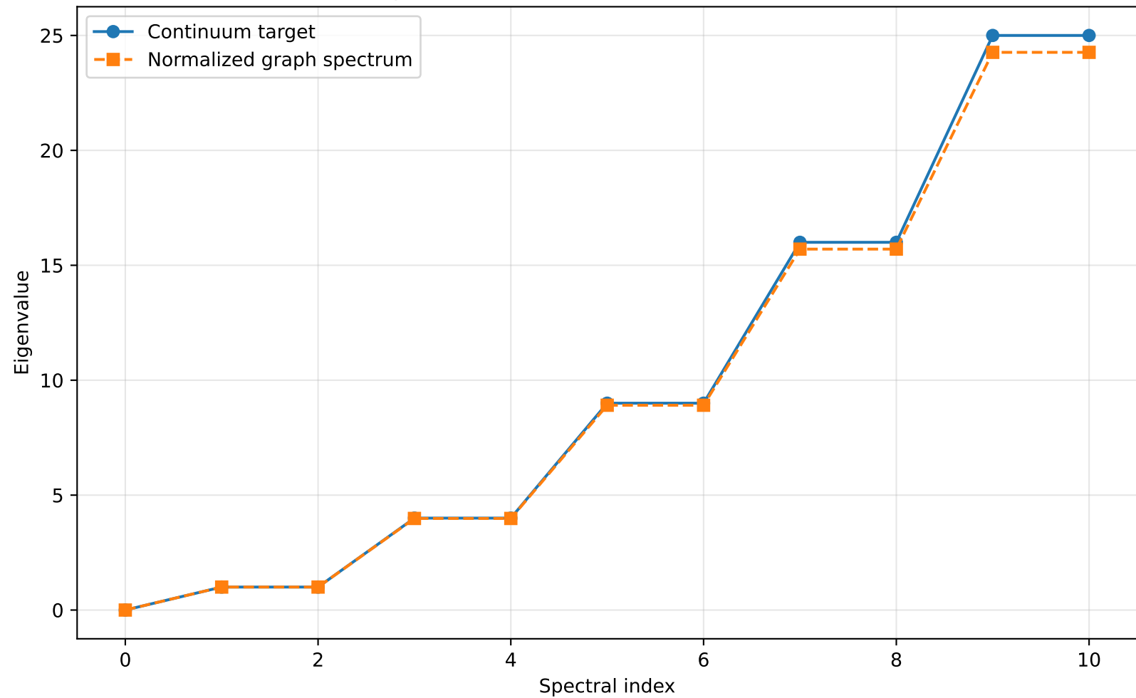
Circle spectrum convergence N=256, epsilon=0.0025, mean relative error=1.232e-02
