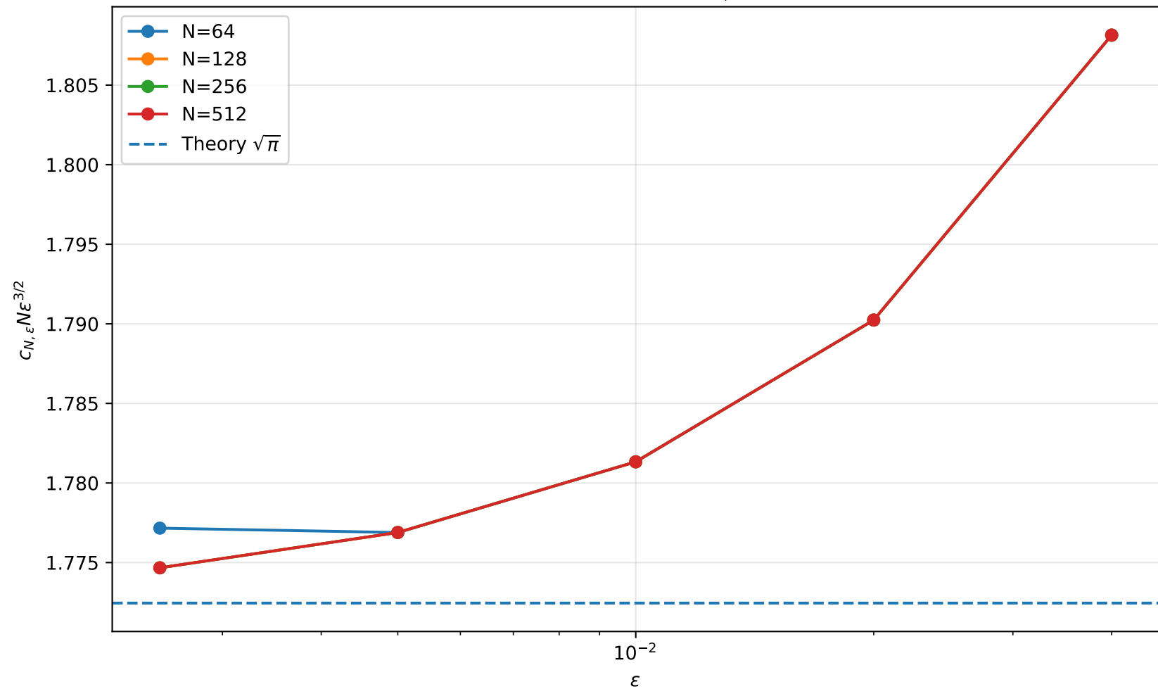
S1 prefactor verification: c_{N,\varepsilon} N \varepsilon^{3/2} \rightarrow \sqrt{\pi}
