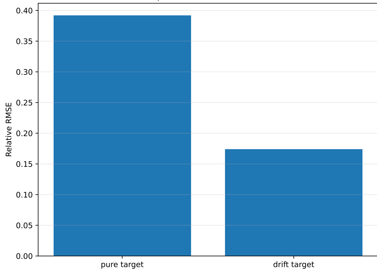
Operator comparison: pure Laplacian vs density-drift target improvement factor = 2.26
