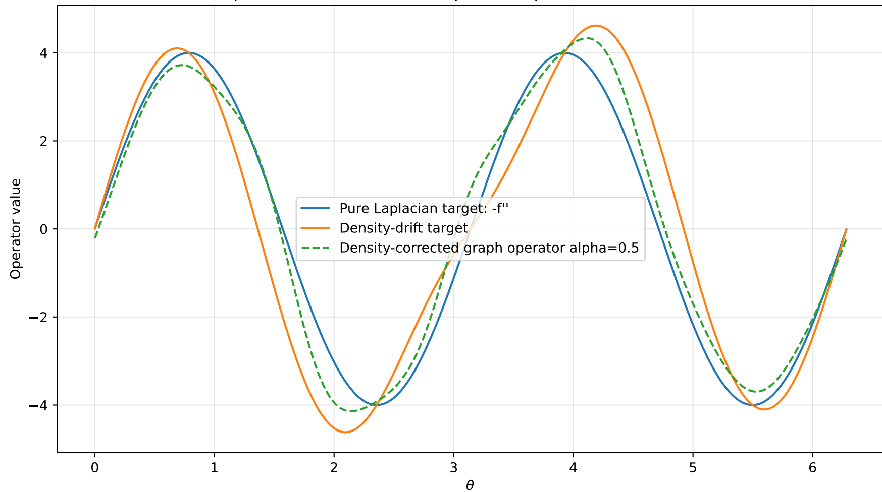
Density-corrected S1 operator compared to pure Laplacian epsilon=0.04, seed=11.0, alpha=0.5, pure RMSE=1.610e-01
