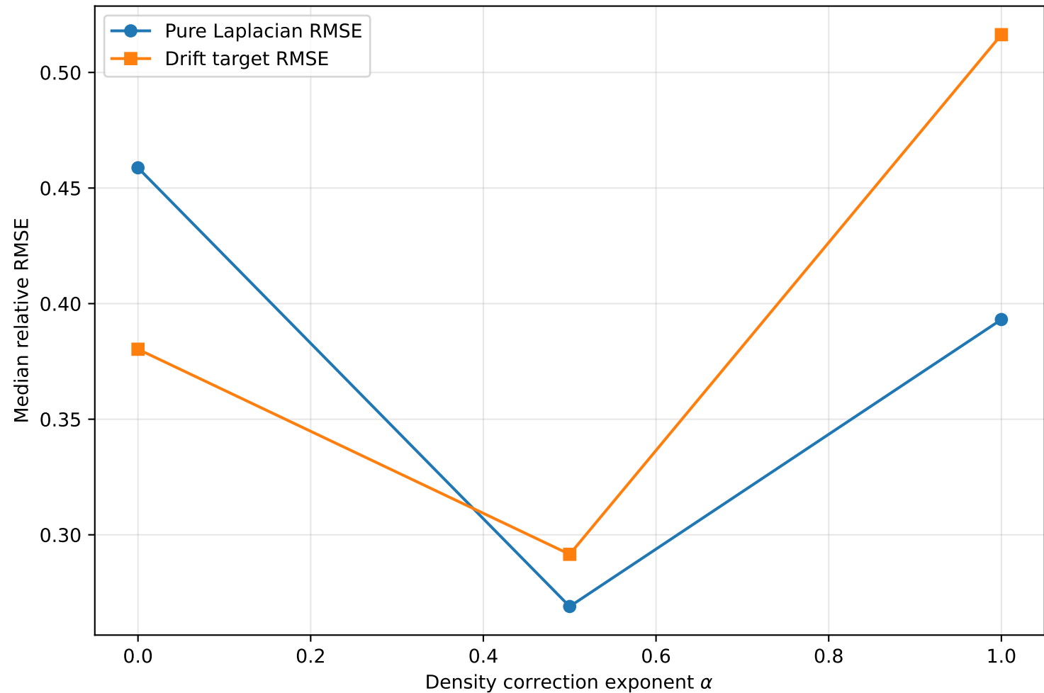
Density correction reduces bias toward the drift operator
