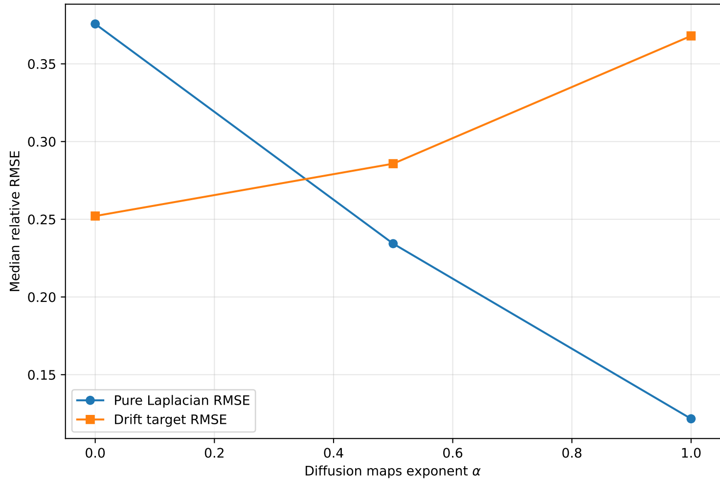
Diffusion-maps Markov generator on non-uniform S1
