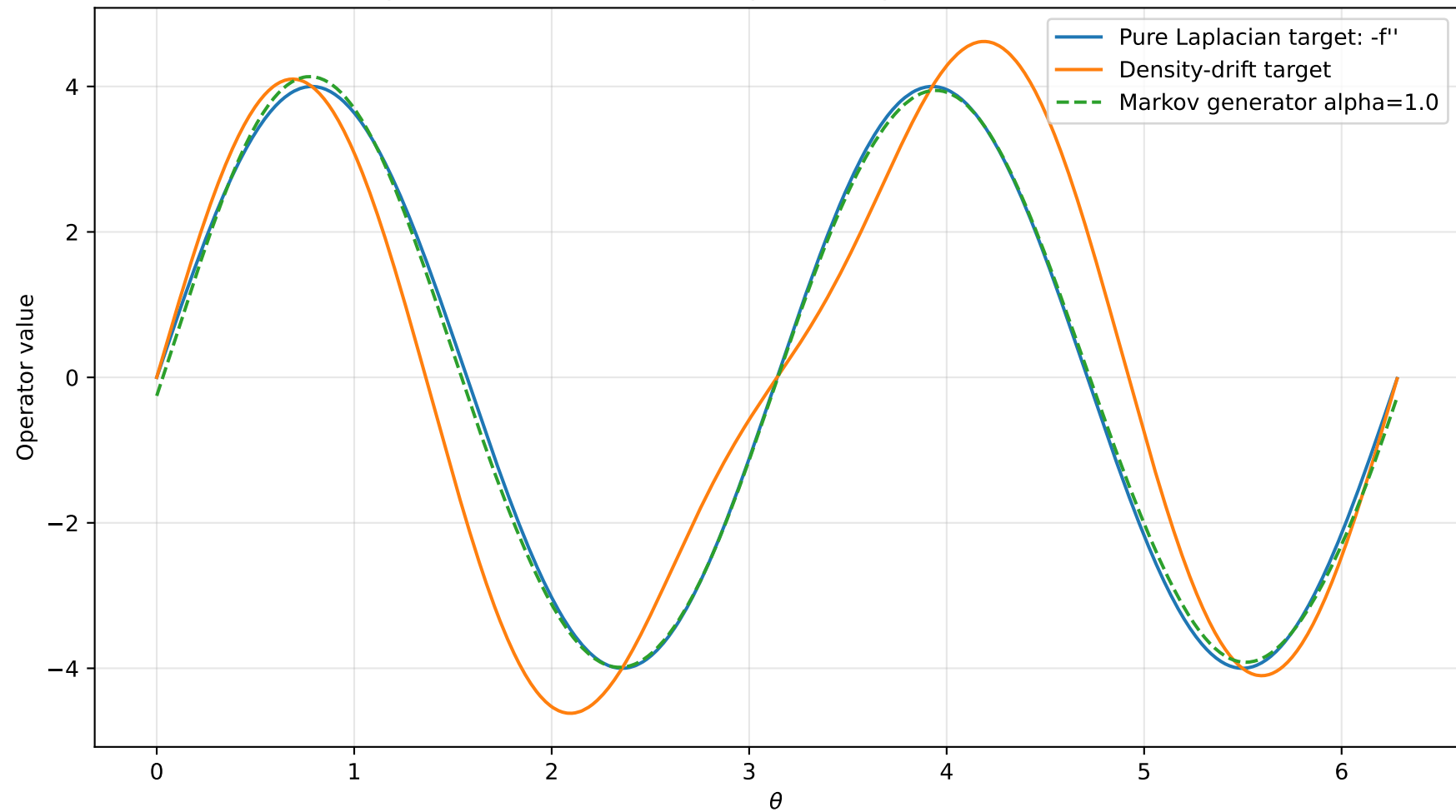
Best diffusion-maps Markov generator recovery epsilon=0.08, seed=33.0, alpha=1.0, pure RMSE=4.406e-02
