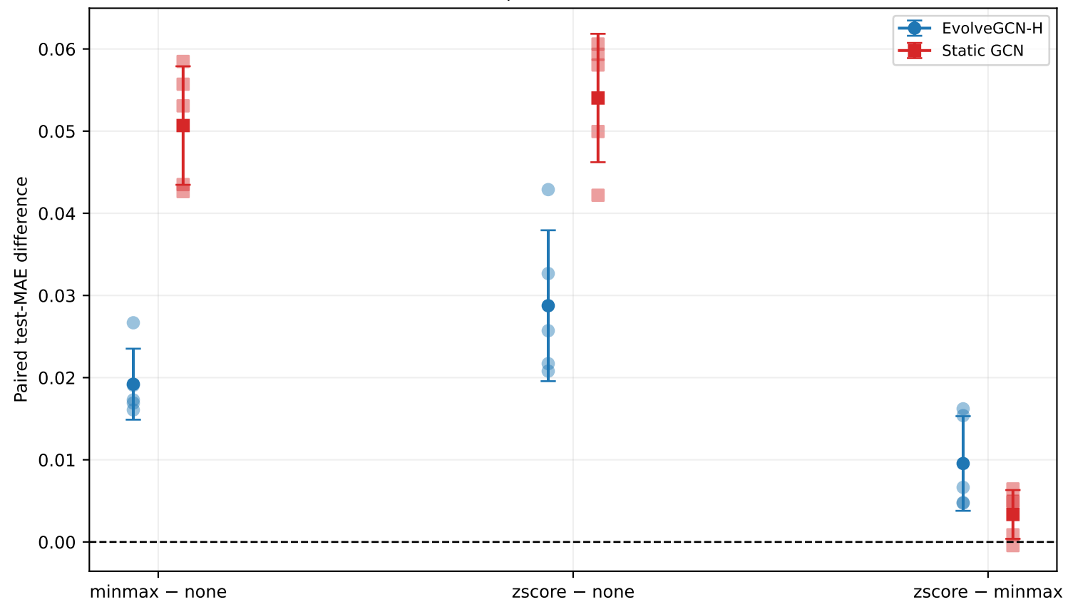
Within-model paired normalization effects
