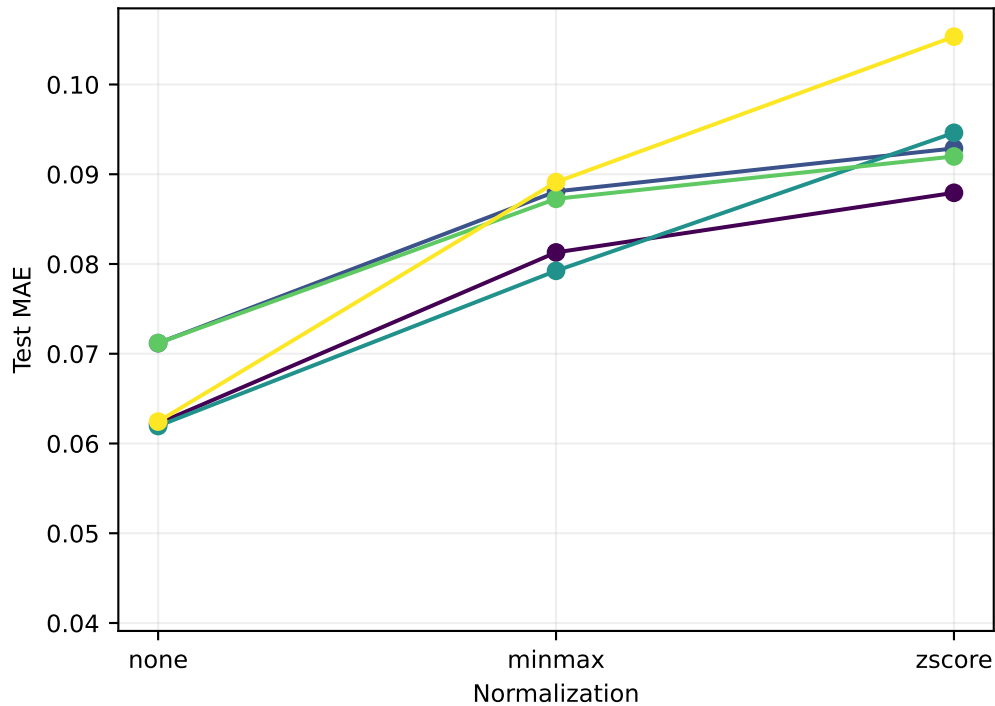
EvolveGCN-H
