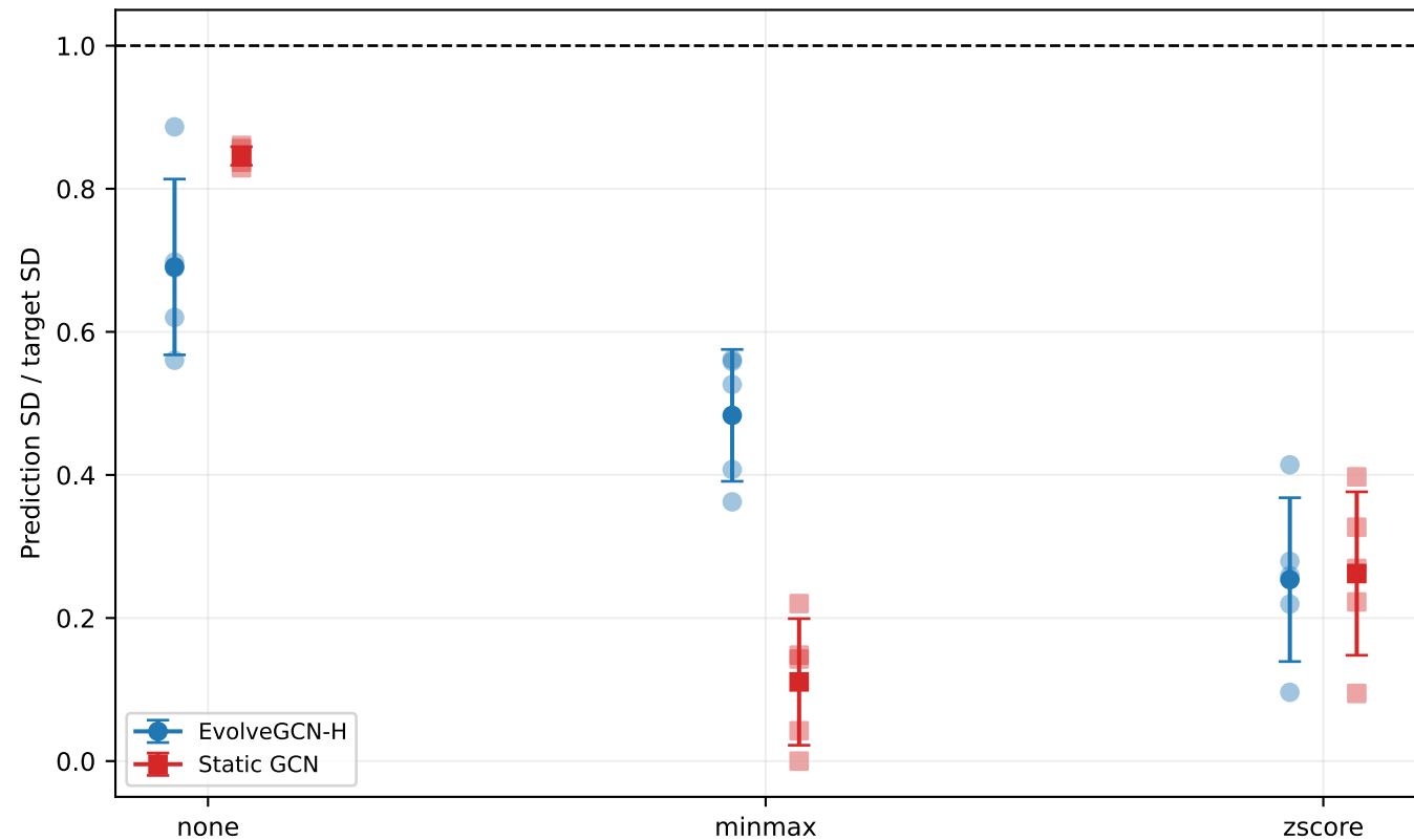
Prediction SD / target SD versus normalization
