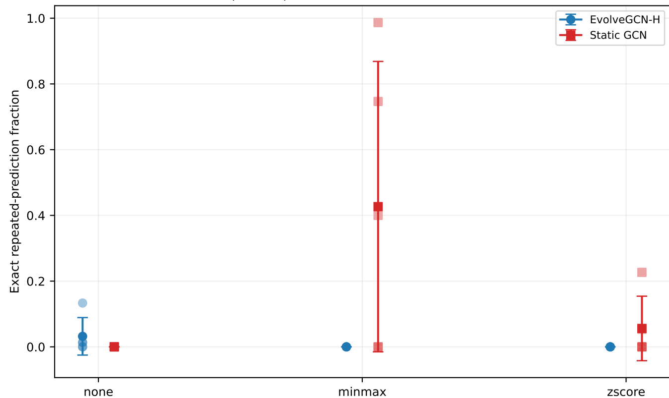
Exact repeated-prediction fraction versus normalization
