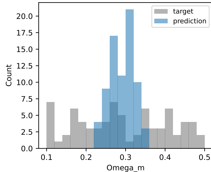
Static GCN, zscore, seed 777
