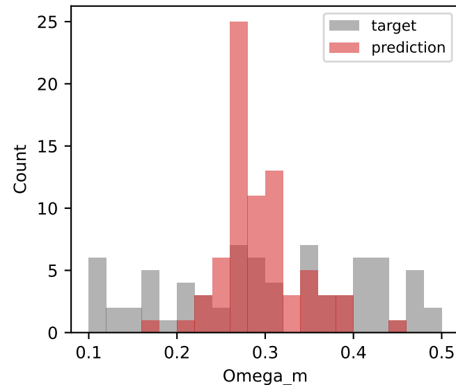
Static GCN, zscore, seed 777
