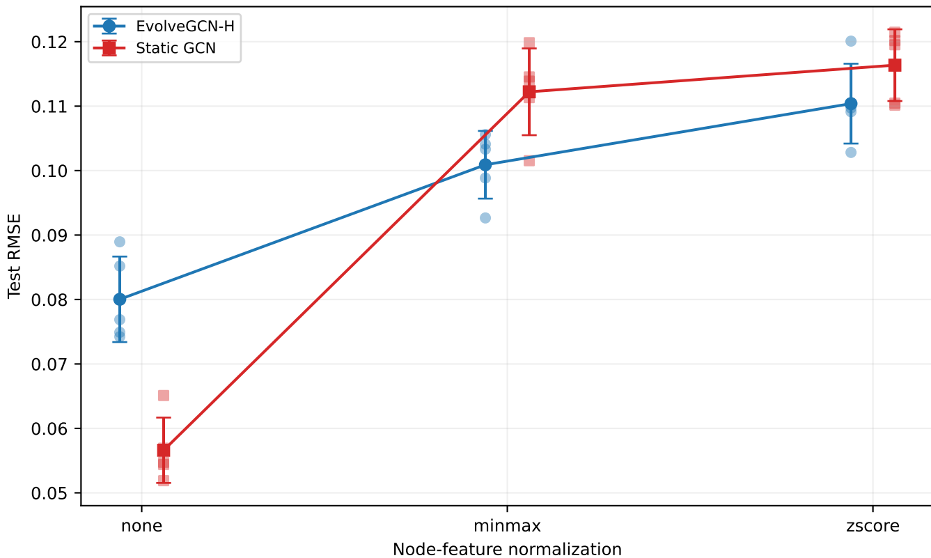
Test RMSE versus normalization
