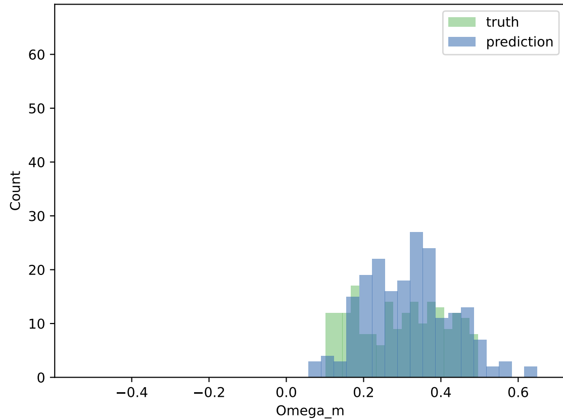
mean, median-MAE seed 123
