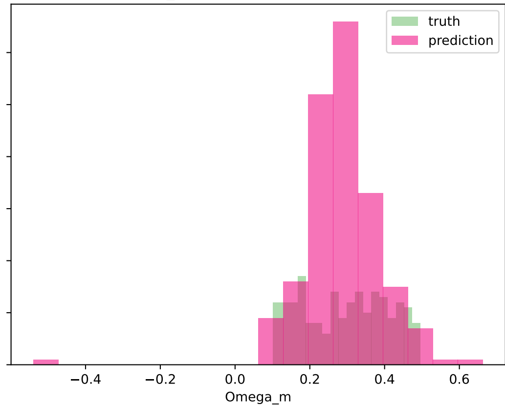
mean_max, median-MAE seed 123
