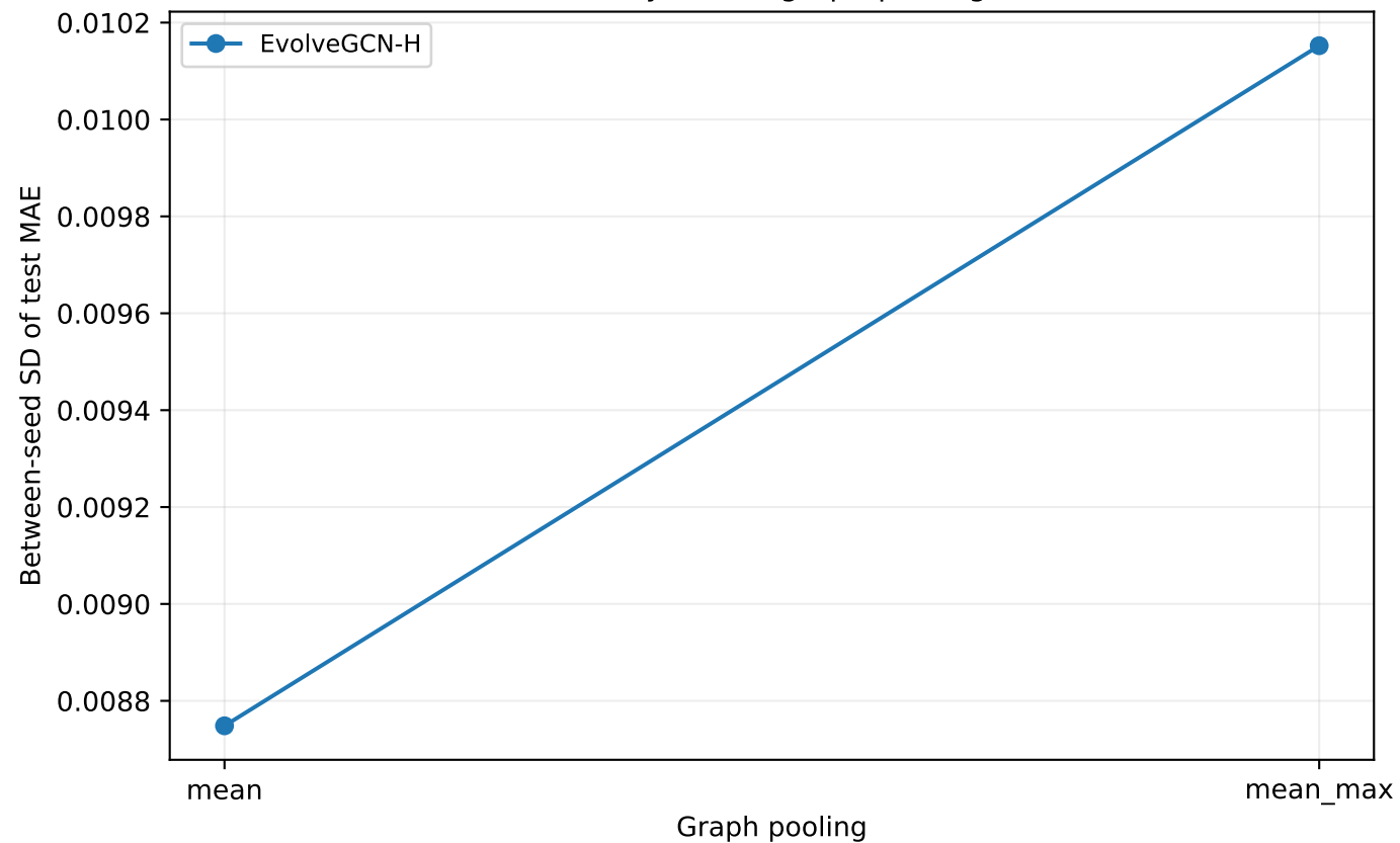
Seed variability versus graph-pooling method
