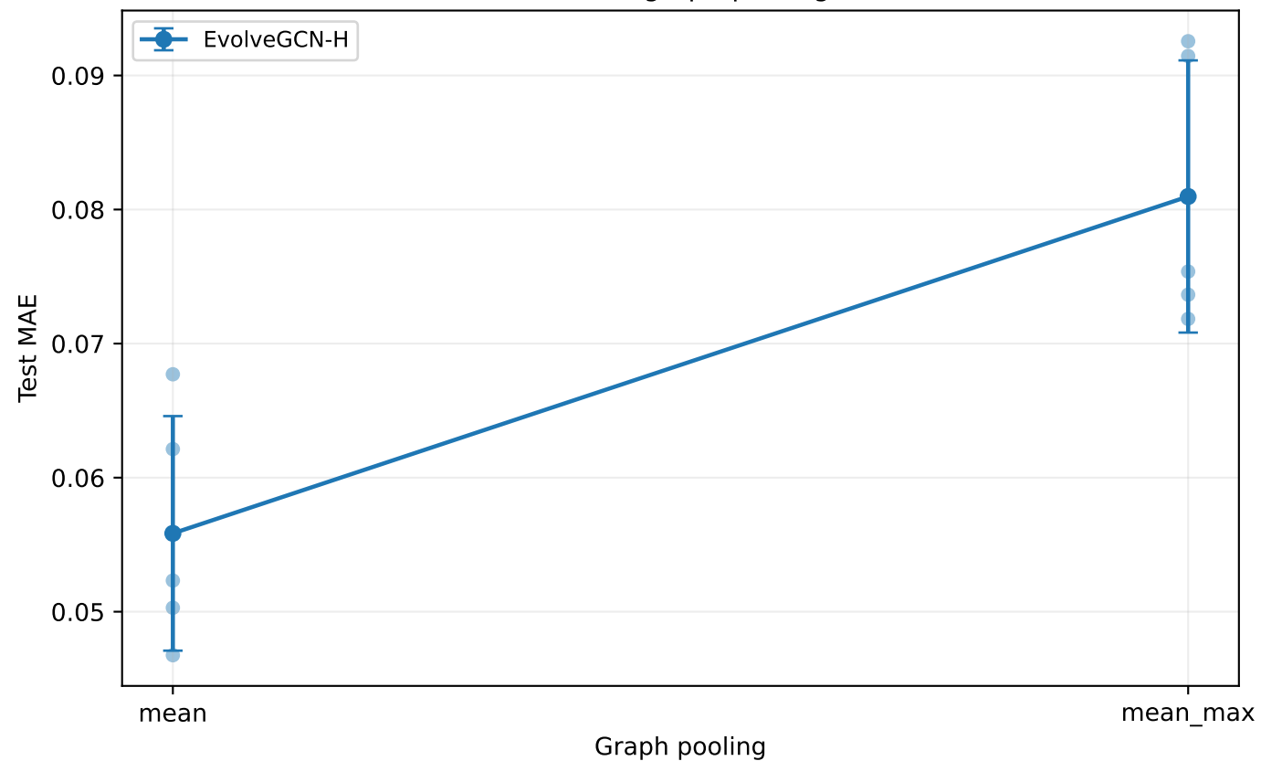
Test MAE versus graph-pooling method
