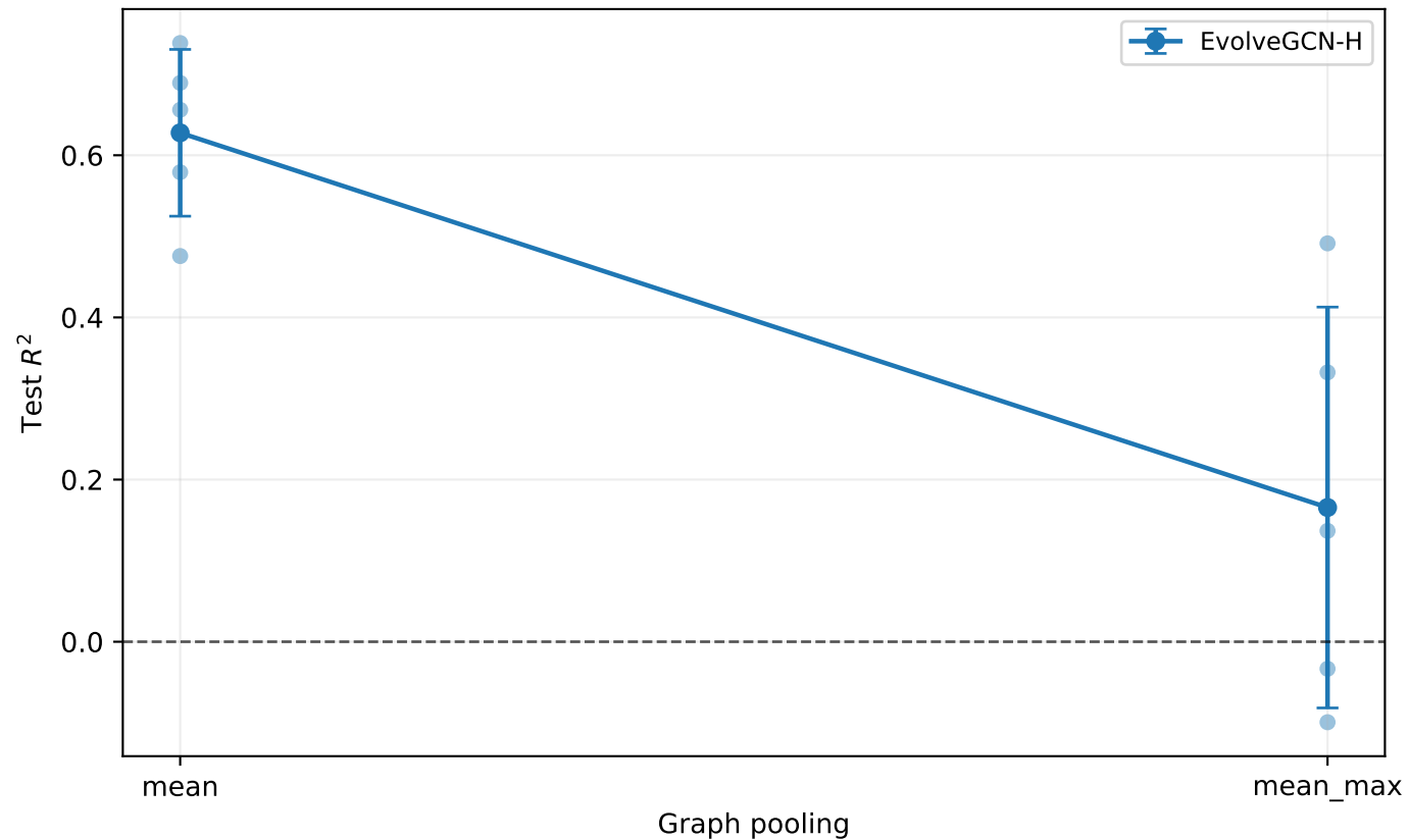
Test R^2 versus graph-pooling method
