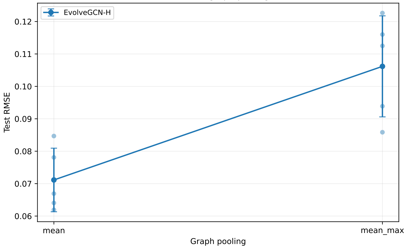
Test RMSE versus graph-pooling method
