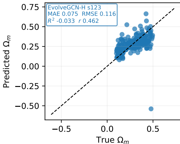
mean_max graph-pooling method
