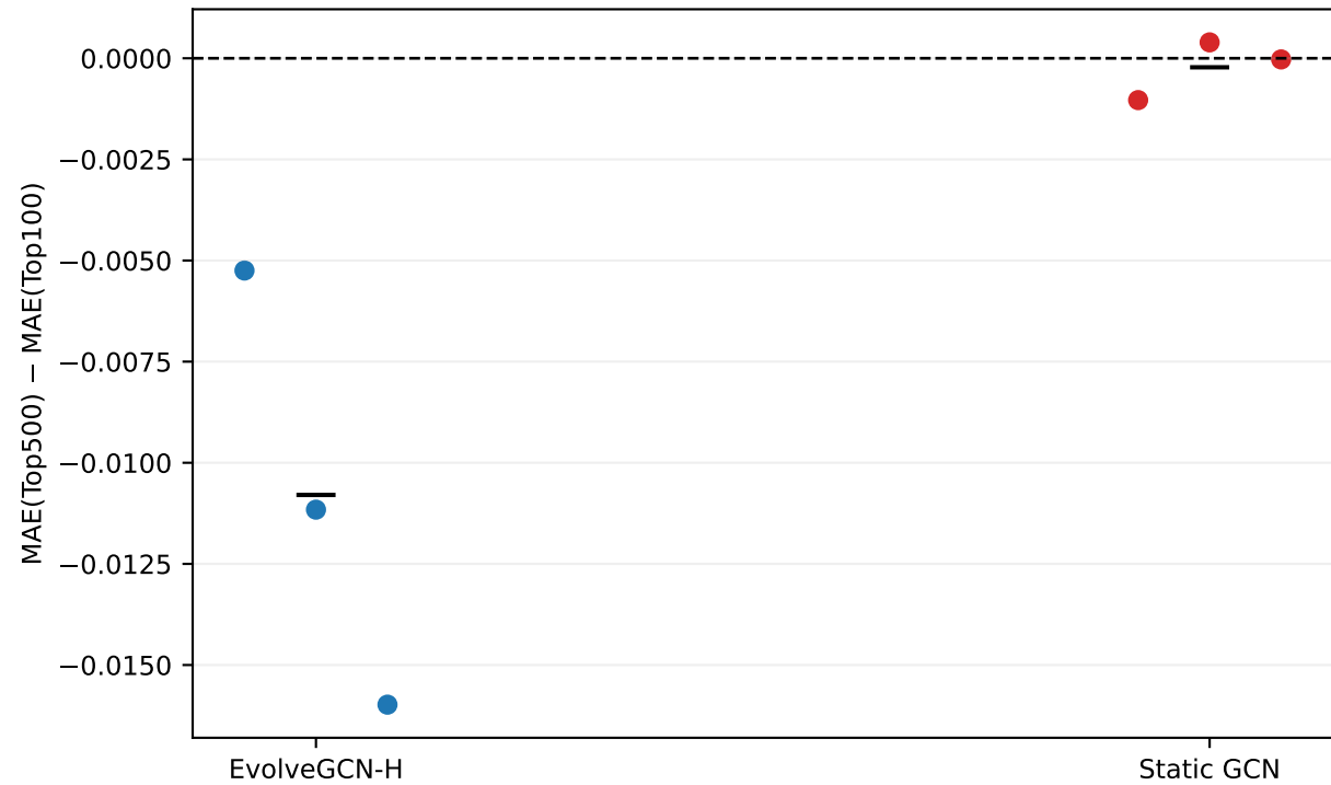
Paired Top500 minus Top100 MAE
