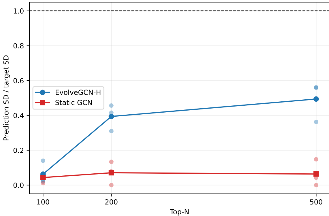
Prediction SD / target SD versus Top-N
