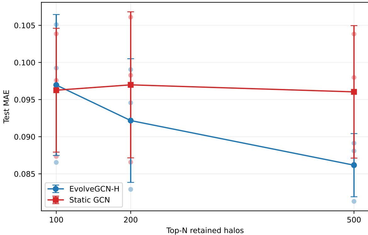
Test MAE versus Top-N
