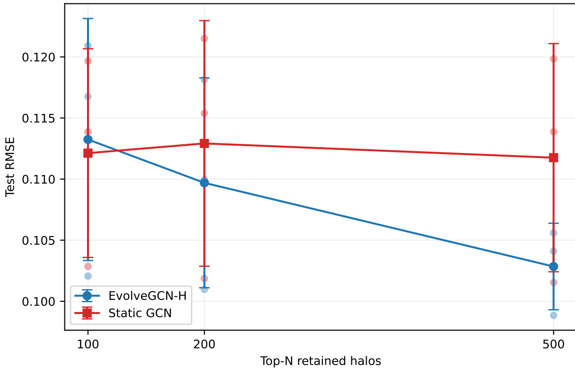
Test RMSE versus Top-N
