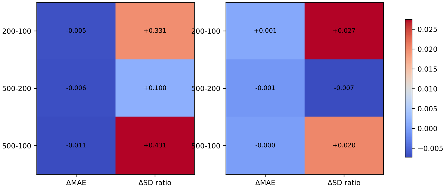
EvolveGCN-H
