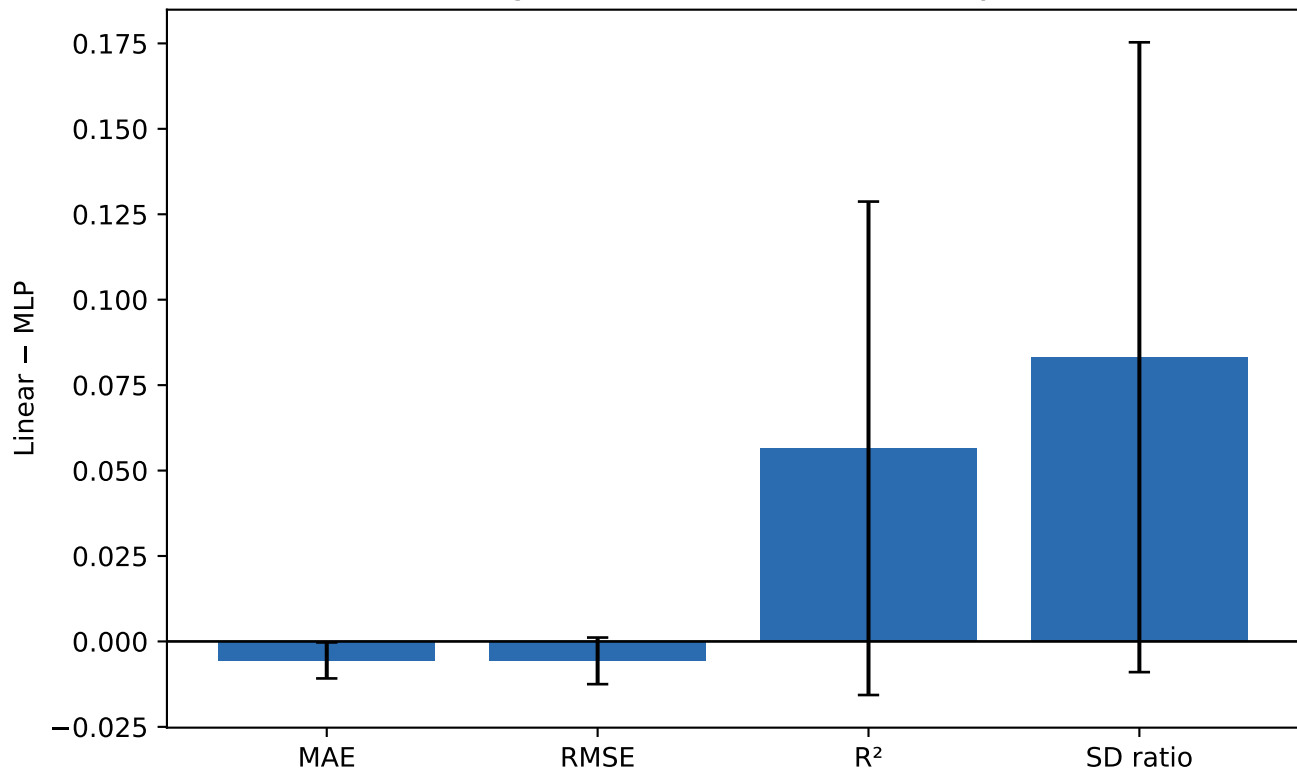
Regression-head effect summary
