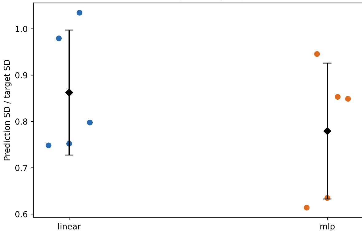
Prediction SD / target SD by regression head
