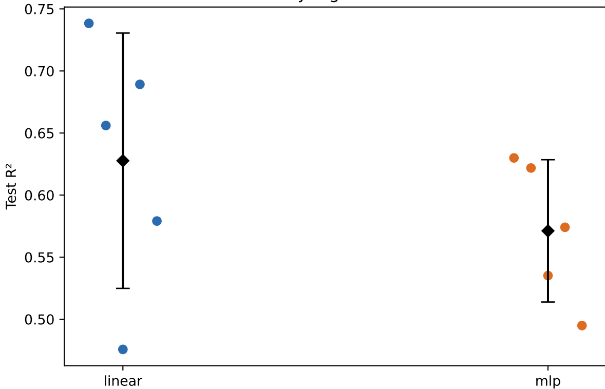
Test R^2 by regression head
